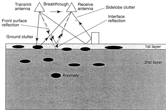
Figure 4. Physical layout of Ground Penetrating Radar system (after Daniels (2004) © IET, 2004).
