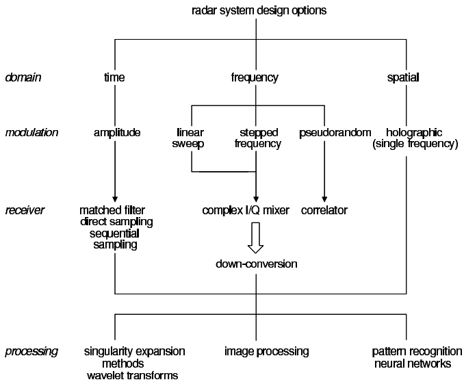
Figure 3. System design and processing options for Ground Penetrating Radar (after Daniels (2004) © IET, 2004).
