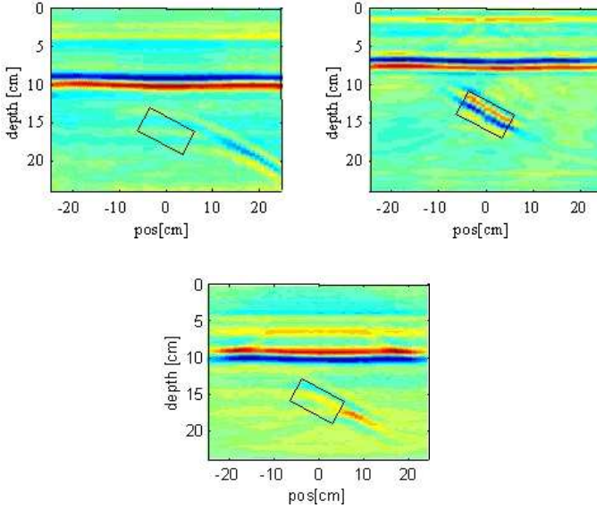
Figure 5. Oblique antipersonnel mine at an angle of 30^\circ : (a) B-scan of raw data; (b) after migration by deconvolution; (c) after Kirchhoff migration (after Daniels (2004) © IET, 2004).
