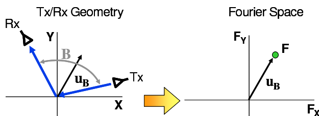
Figure 7. Relationship between bistatic sensor geometry and representation in Fourier space (after Bonneau et al. (2002)).
