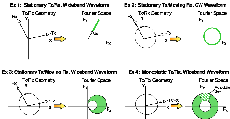
Figure 9. Fourier space sampling and scene resolution for four examples: (i) stationary tx/rx, wideband waveform; (ii) stationary tx, moving rx, CW waveform; (iii) stationary tx, moving rx, wideband waveform; (iv) monostatic tx/rx, wideband waveform (after Bonneau et al. (2002)).
