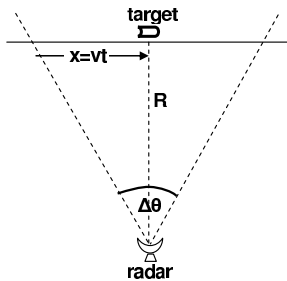
Figure 1. A target moving perpendicularly past a monochromatic CW radar.
