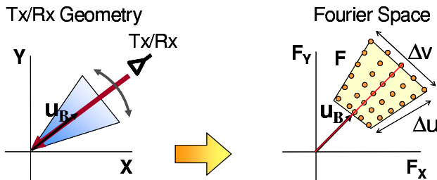
Figure 8. Fourier space sampling and scene resolution for a monostatic SAR (after Bonneau et al. (2002)).
