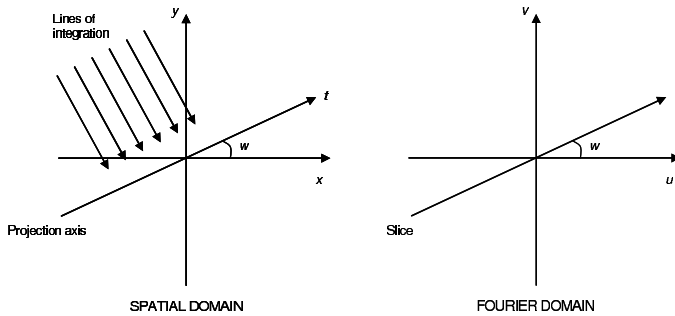
Figure 6. Tomographic reconstruction: the Projection Slice Theorem.
