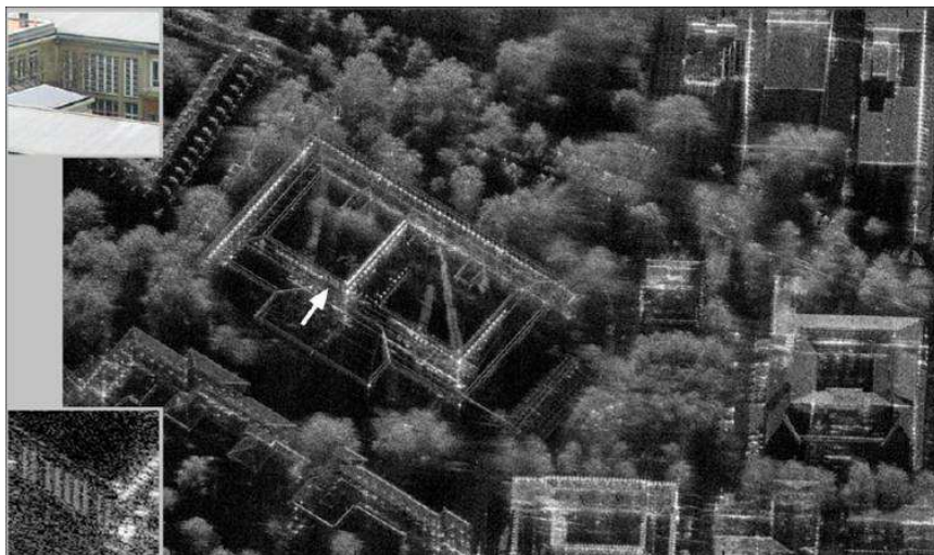
Figure 2. High resolution aircraft-borne SAR image of a part of the university campus in Karlsruhe (Germany). The white arrow refers to a lattice in the left courtyard, which is shown in more detail in the small picture on the left bottom. The corresponding optical image is shown on the left top (after Brenner and Ender (2004)).
